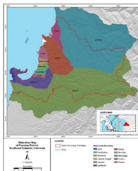
Figure 3. Watershed Map of Pomalaa District
