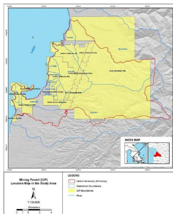
Figure 4. Location Map of Mining Permits and Watersheds in Pomalaa District Impact of Nickel Mining Activities on Watershed Hydrology and Coastal Sedimentation
