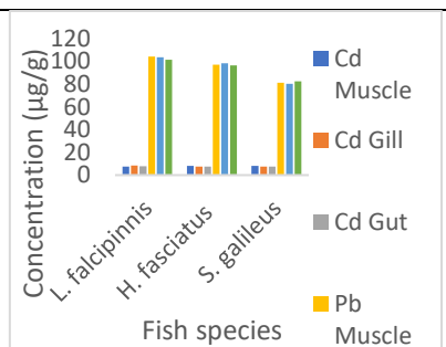
Figure 15. Concentrations of Cd and Pb in Fish Tissues from Ilelema, Buguma Creek, Rivers State, Apr., 2020
