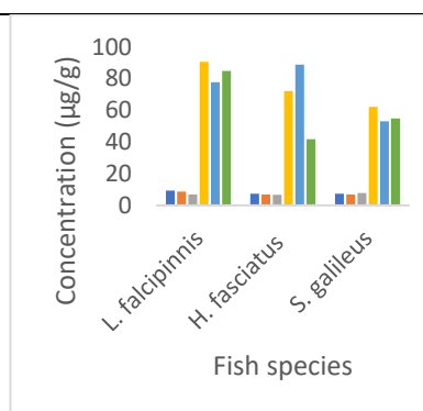
Figure 8. Concentrations of Cd and Pb in Fish Tissues from Abalama, Buguma Creek, Rivers State, Mar., 2020
