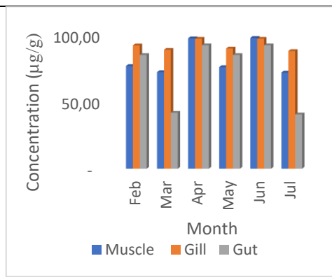
Figure 5. Monthly variation of Cd in H. fasciatus of Ilelema, Buguma Creek, Rivers State, Nigeria
