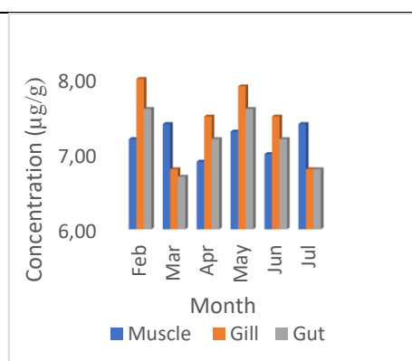
Figure 2. Monthly variation of Cd in H. fasciatus of Abalama, Buguma Creek, Rivers State, Nigeria
