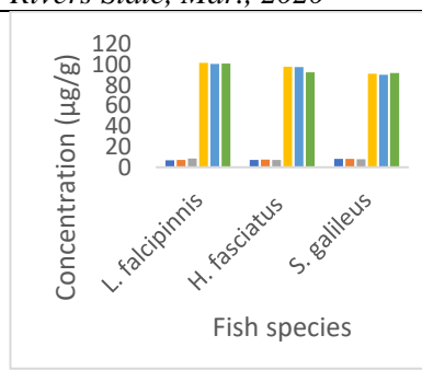
Figure 11. Concentrations of Cd and Pb in Fish Tissues from Abalama, Buguma Creek, Rivers State, Jun., 2020
